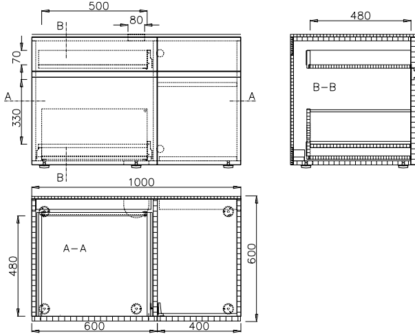
K 41 Container with equipment extension
