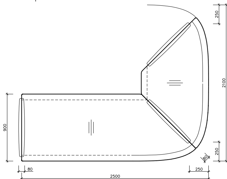
V 66 Head top
