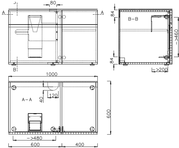
K 40 Container with PC-fitting
