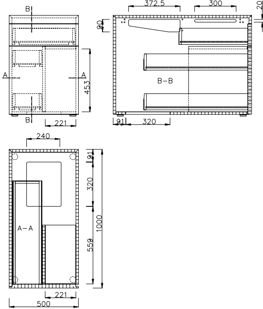
246 / 247 CPU-Container
