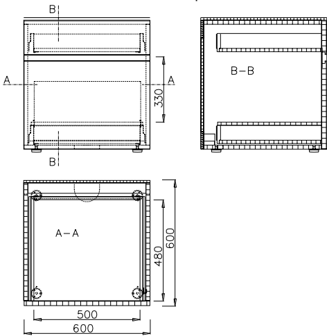
K 46 Container with drawer for printer
