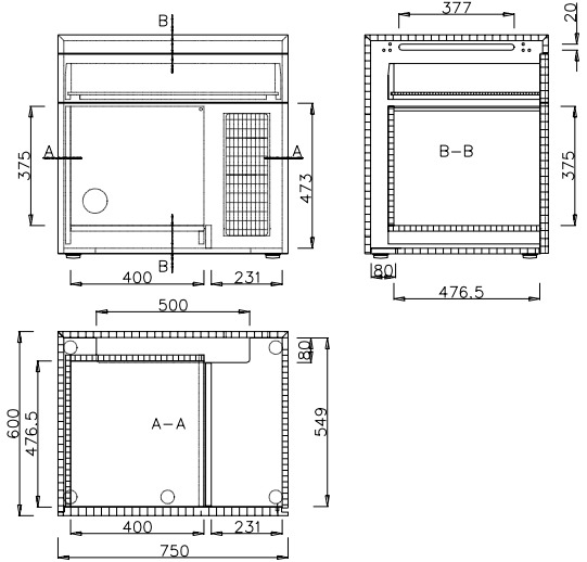
264 / 265 CPU-Container
