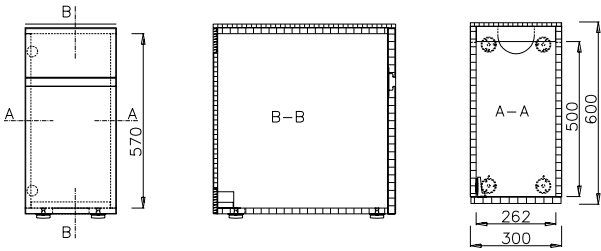
K 48 Container for PC
